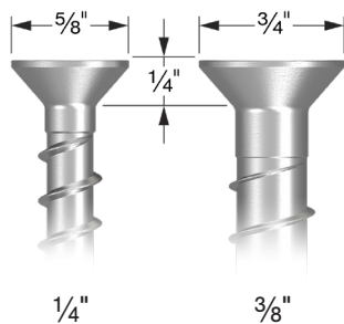
Countersunk Head Dimensions
